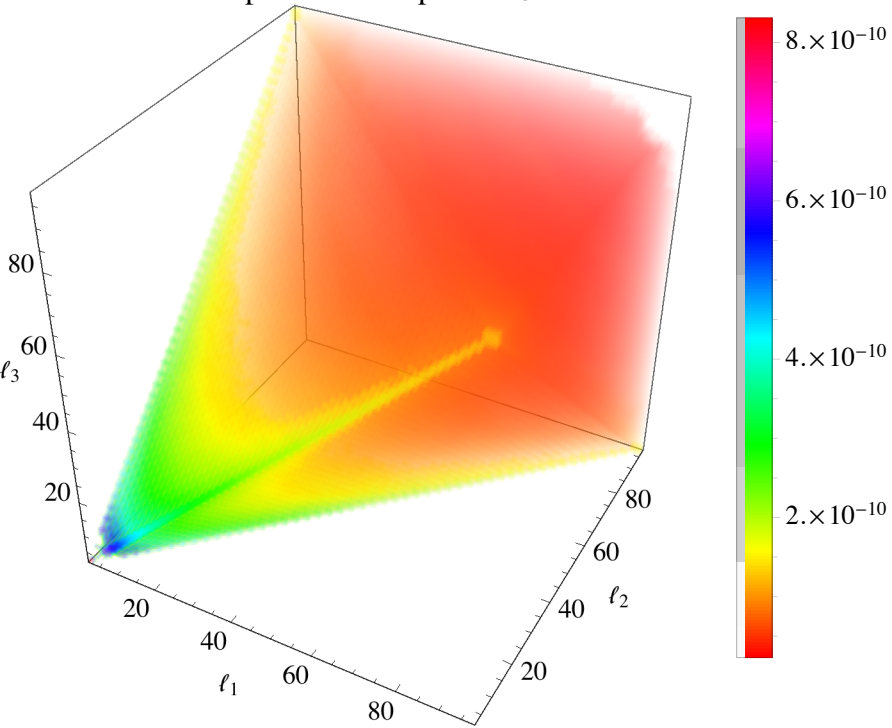
Local template in \ell m -space at z=0.55
